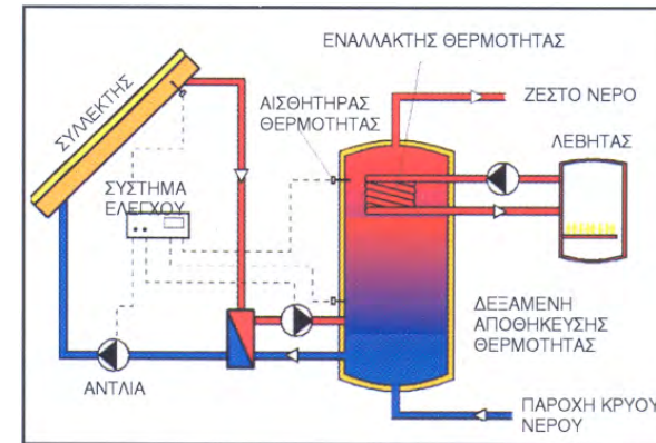
SOLAR COLLECTOR
