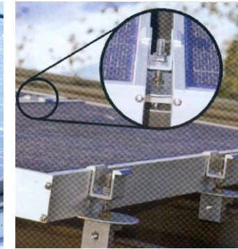
PHOTOVOLTAIC PANELS
