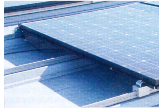
PHOTOVOLTAIC PANELS
