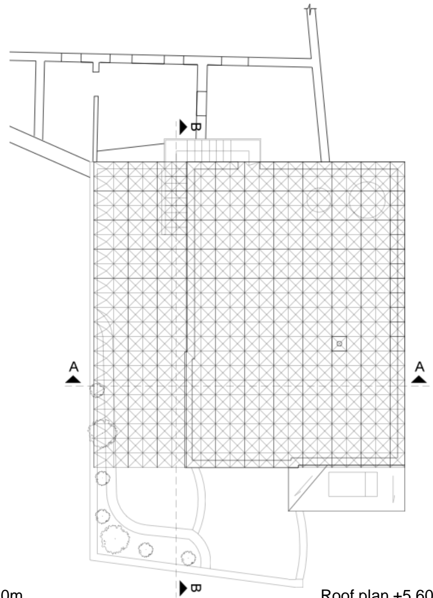
Roof plan +5.60m
