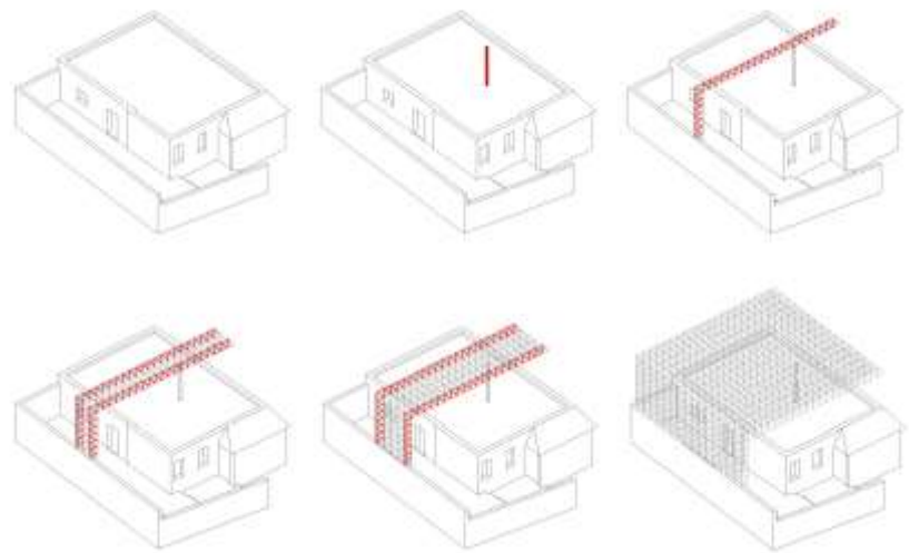
construction phases
